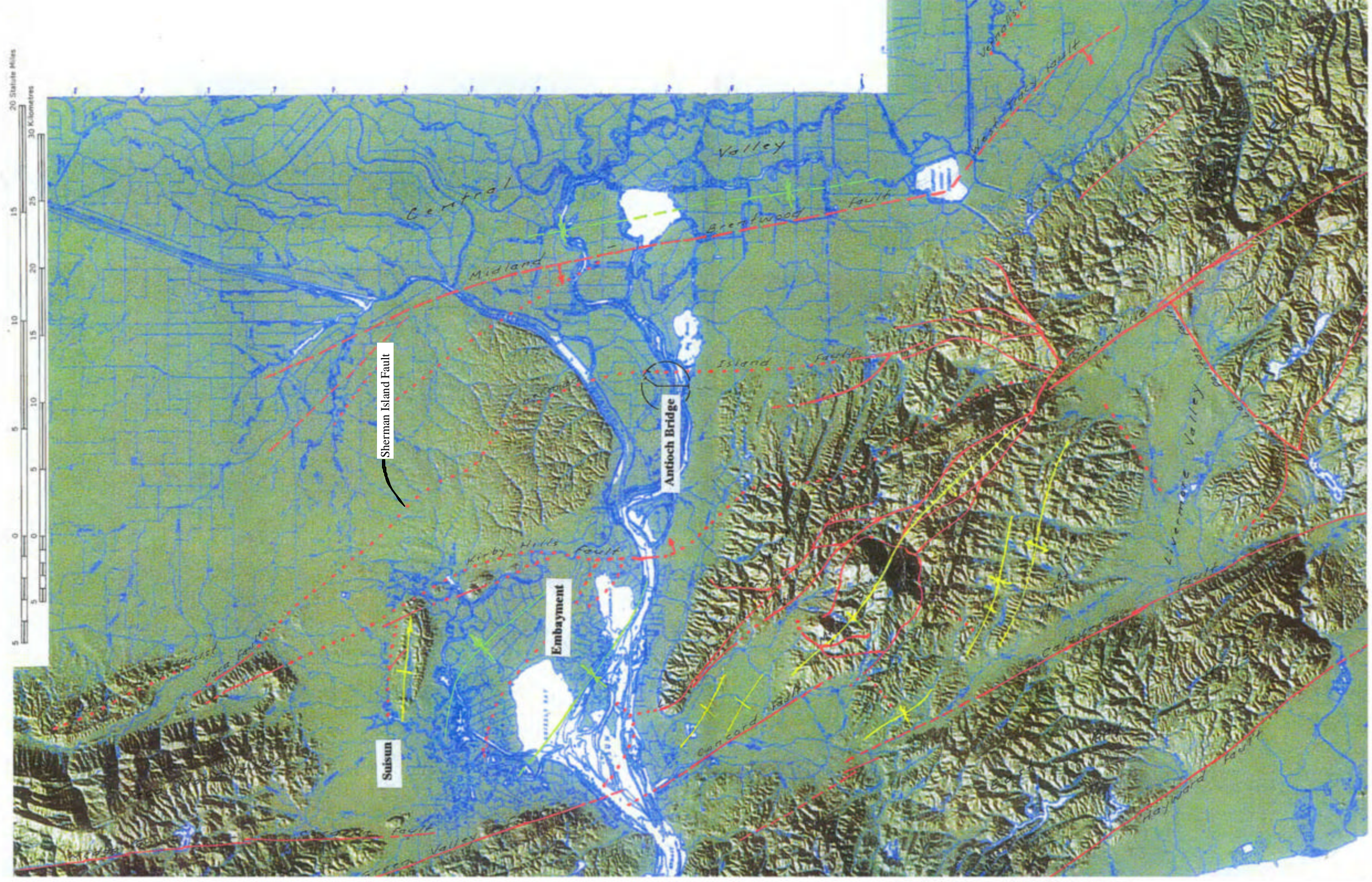
Terrain and Faults, Suisun Embayment and Antioch Area
